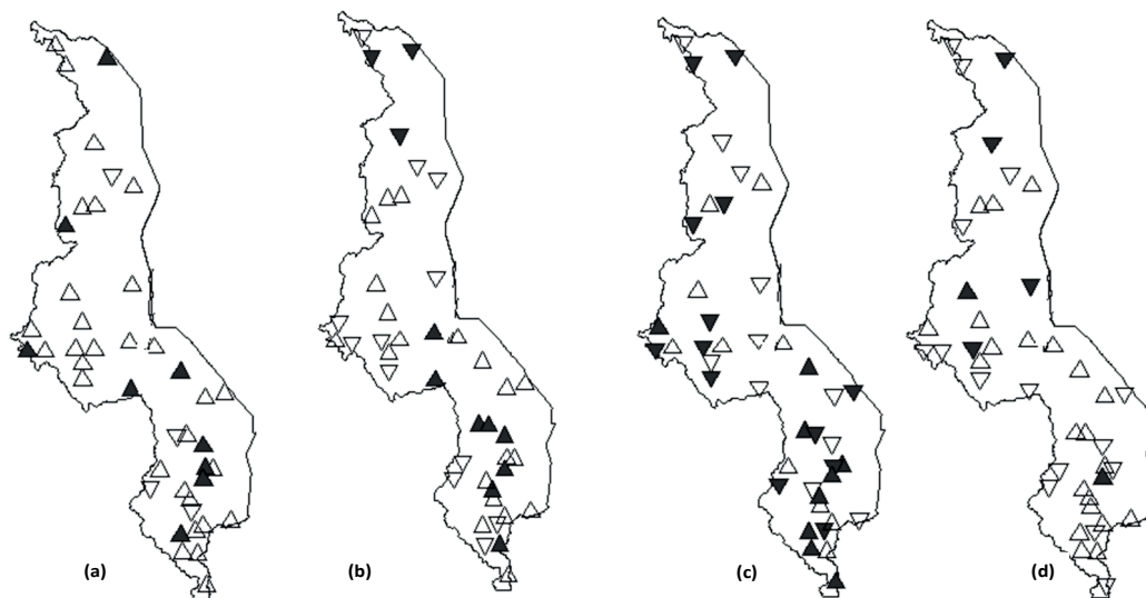
Fig. 3 Mann-Kendall trends in (a) CDD; (b) SDII; (c) Rx5day; and (d) R95p. Positive trends = upward triangle; negative trends = downwards triangles. Statistically significant trend at \alpha = 0.05 level are shaded.
